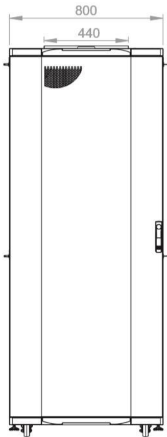
Front view
